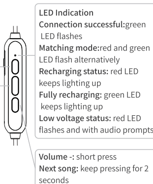
Earphone Diagram
