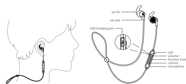
Wearing Diagram
